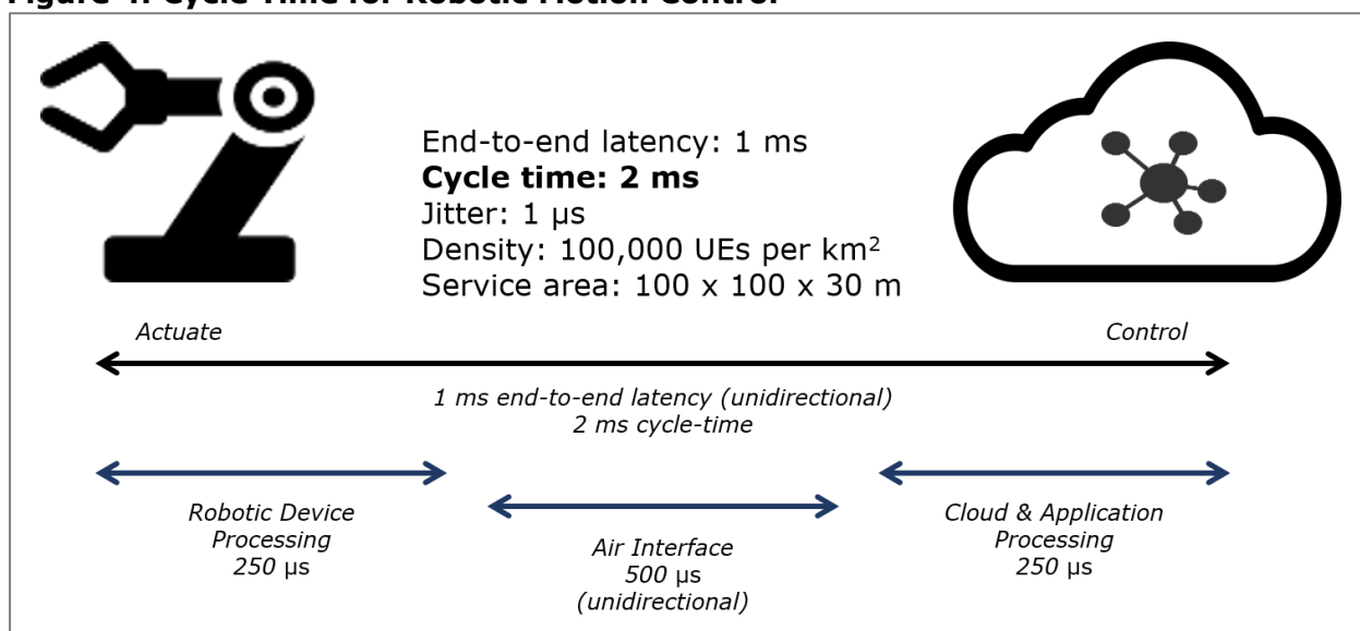
Figure 4: Cycle Time for Robotic Motion Control
