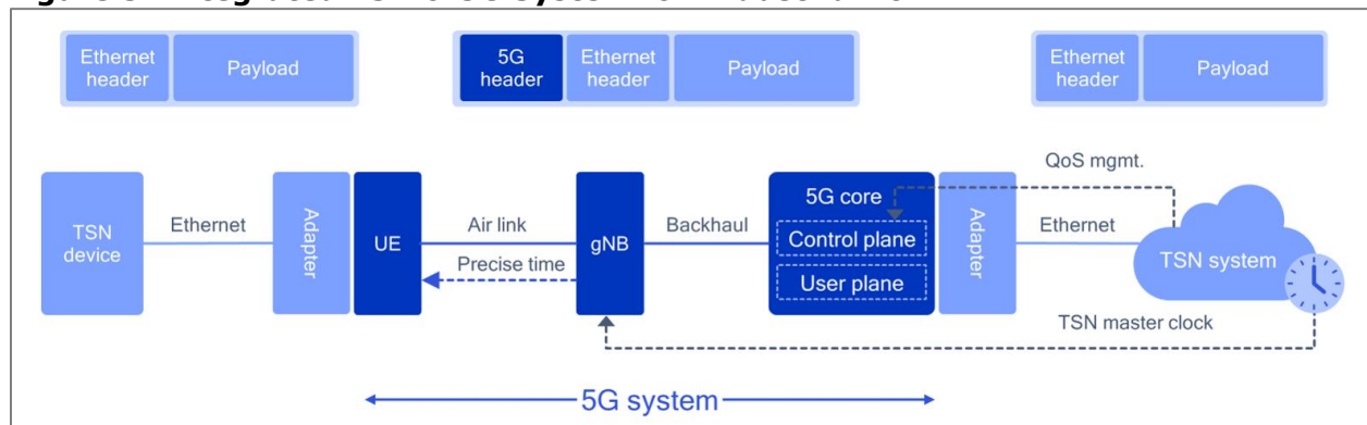
Figure 5: Integrated TSN & 5G System for Industrial IoT
